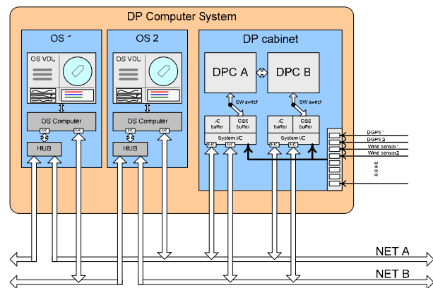
Figure 3: Example of a DP computer system.
