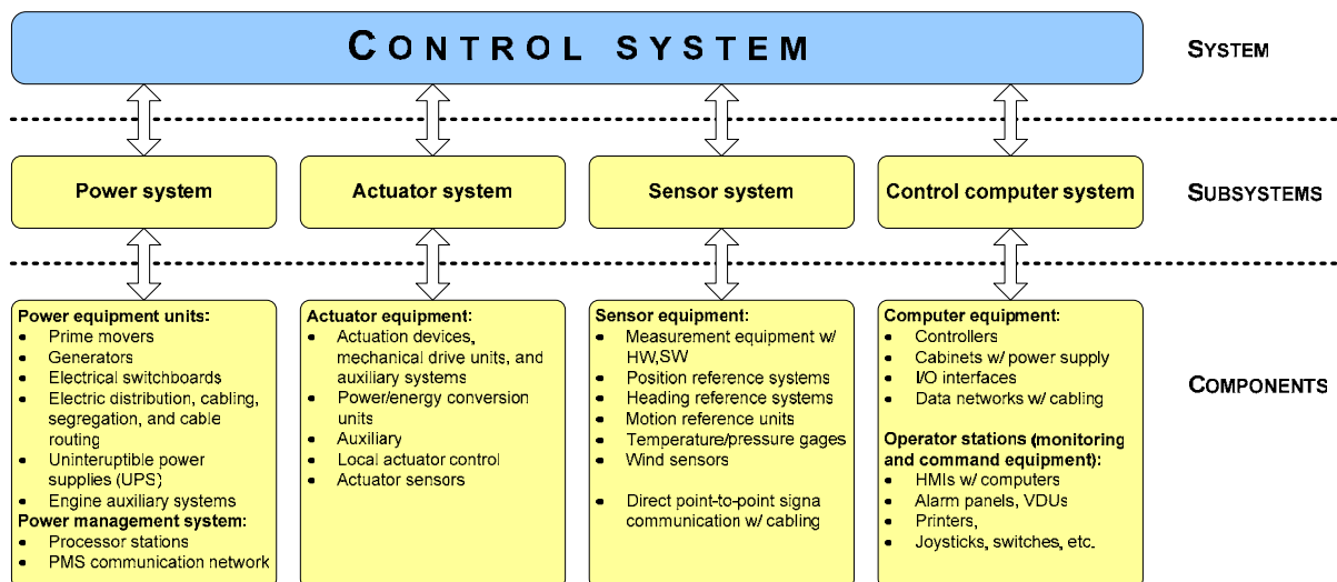
Figure 1: Control system hierarchy.
