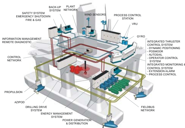
Figure 2: Integrated automation system in a semi-submersible (Courtesy: ABB)
