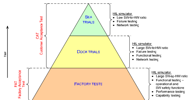
Figure 4: Scope of testing for HIL certification in a new-building project
