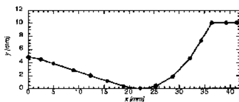
Fig. 4. Silhouette of piston bowl
