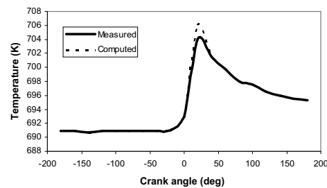
Fig. 7. Surface temperature comparison on the cylinder head for fired engine case
