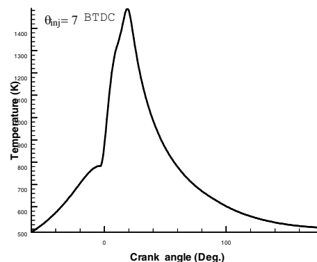
Fig. 2. Cylinder Temperature against crank angle for Isuzu engine
